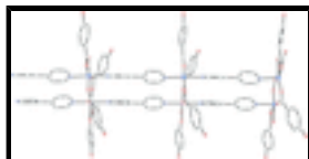
Fig. 2. The 1D double chain in the title complex. Non-coordinated molecules and hydrogen atoms are omitted for clarity.
